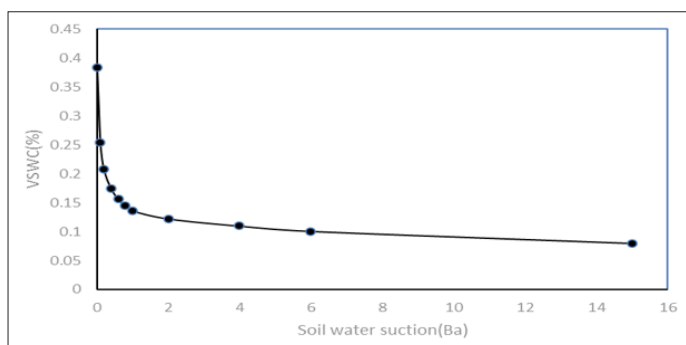
Figure 1: Volume soil water content change with soil water suction.
